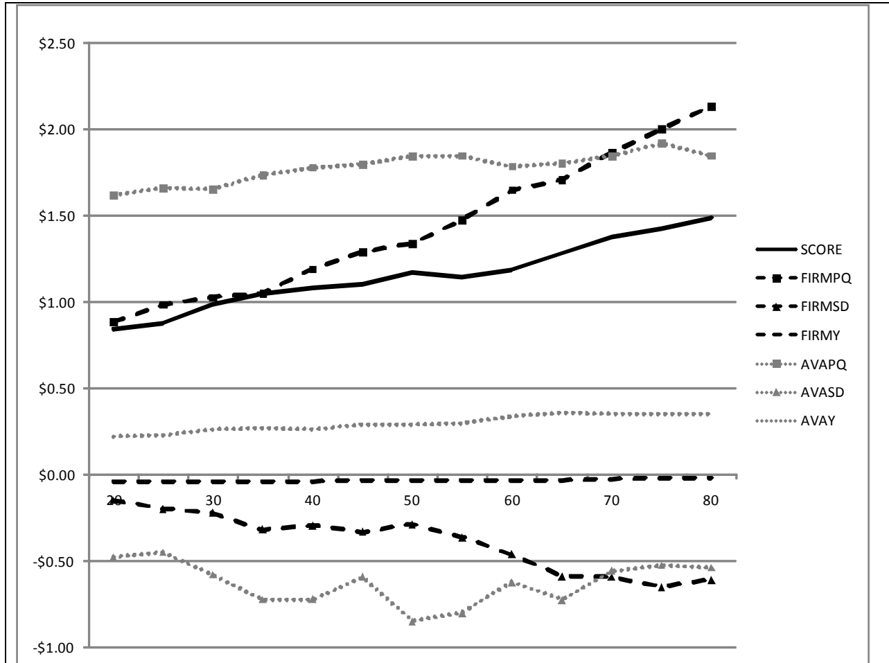
Figure 1: Selected a Estimates for Each 5 th Conditional Quantile \in [20, 80]
